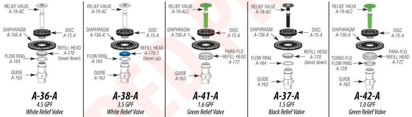
Closets — Diaphragm Inside Parts Kits
