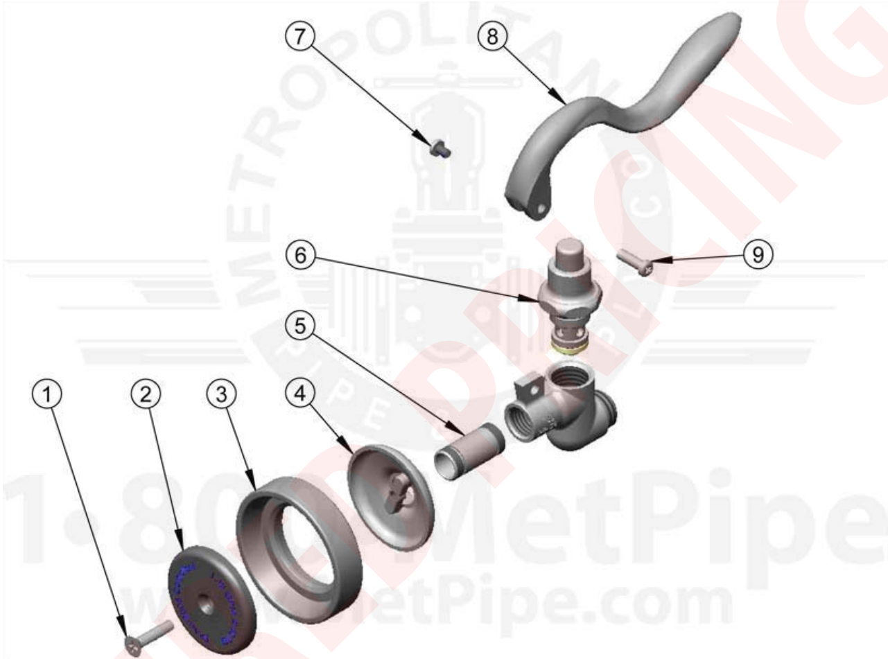
B-0107 Spray Valve
